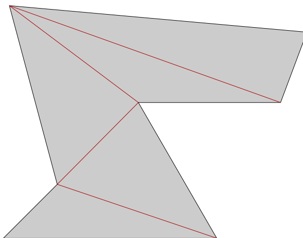
Figure 171: Triangulating a non-convex polygon
